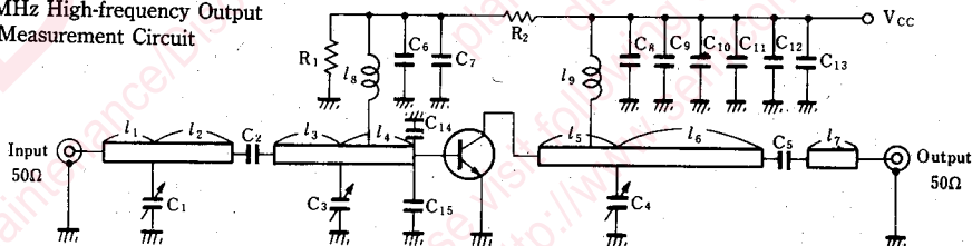
Circuit Fixed Number (Printed Substrate: Glass Epoxy Substrate Et=4.8 t=1.6)
