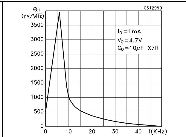
Figure 18. Worst case: lowest output version
