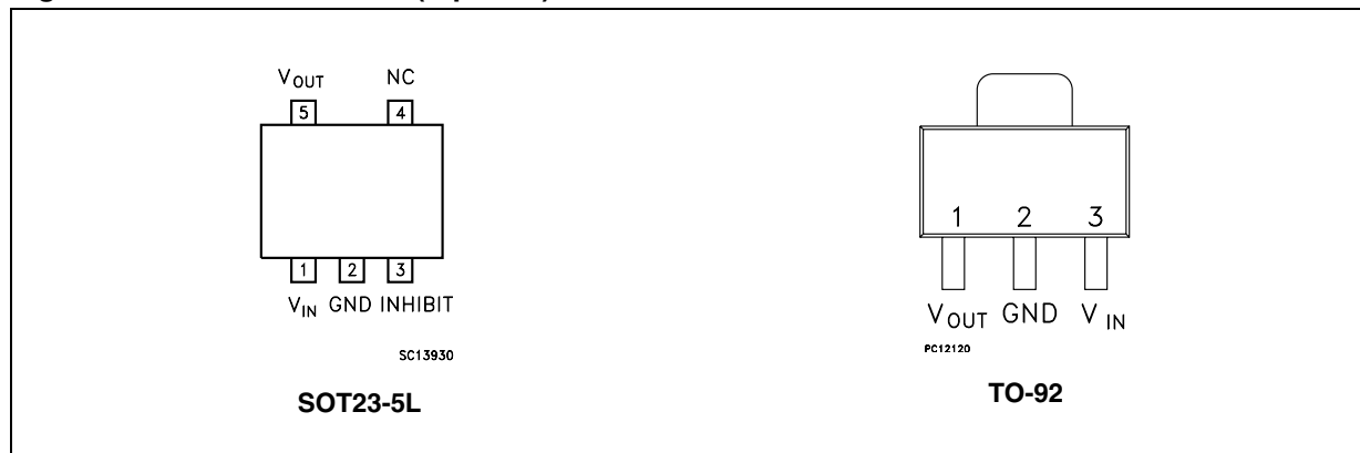
Figure 1. Pin connections (top view)
