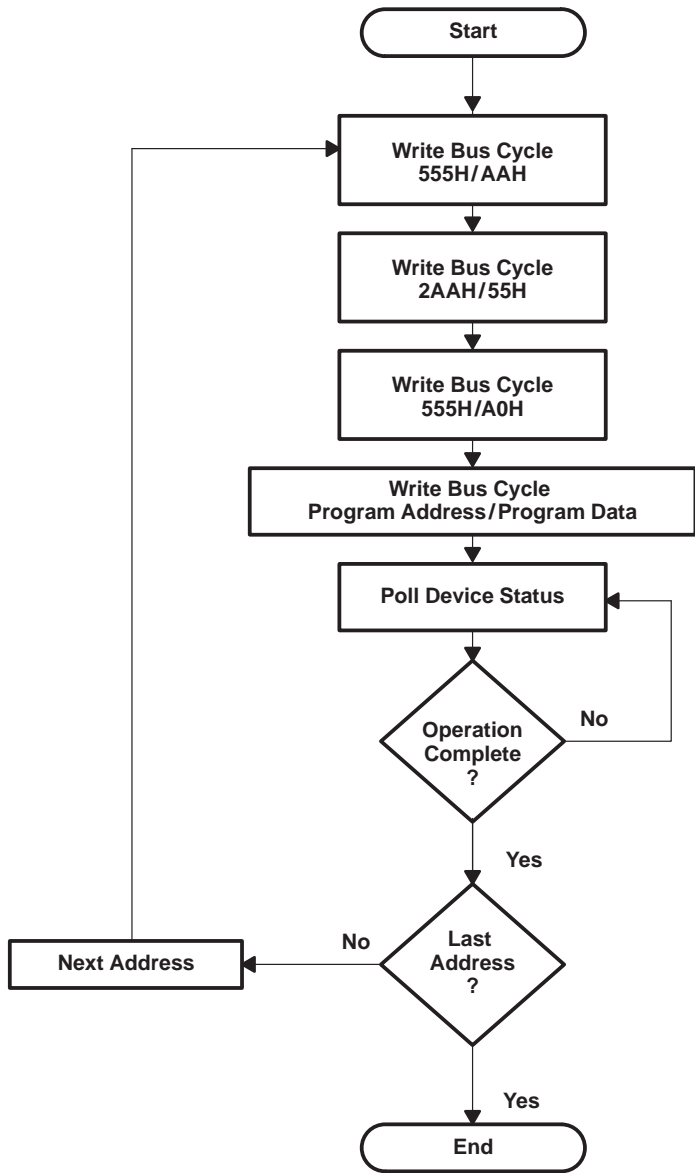
Figure 7. Program Algorithm
