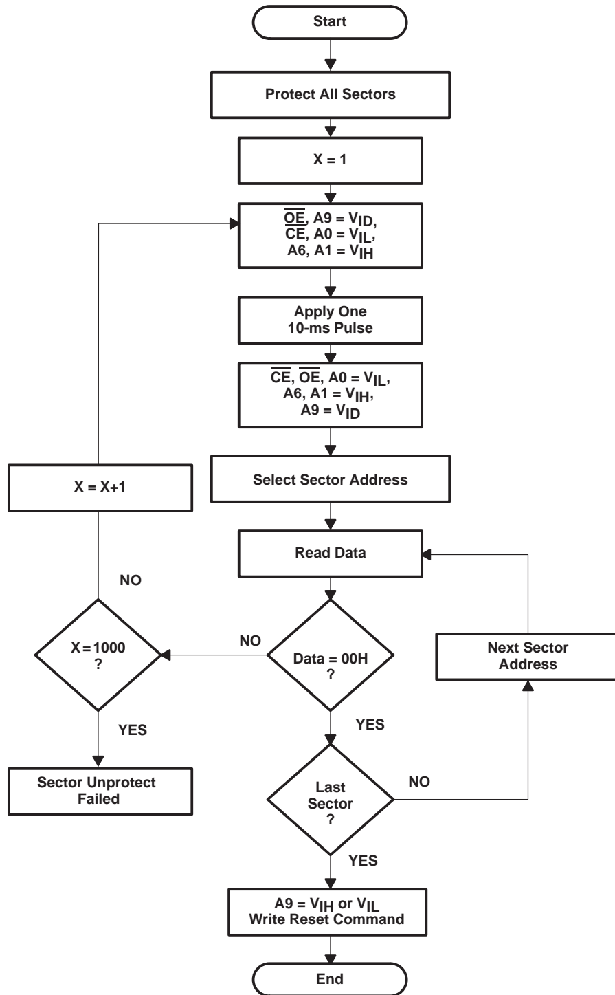
Figure 20. Sector-Unprotect Algorithm
