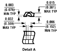
Ceramic Leadless Chip Carrier Package (E) Order Number 54LS192LMQB NS Package Number E20A
