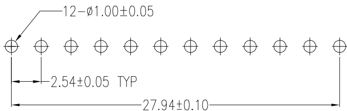
PCB LAYOUT(TOP)
