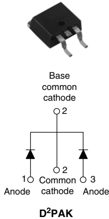
MBRB4045CTPbF
