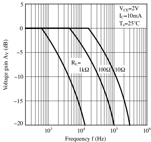
Fig.11 Frequency Response
