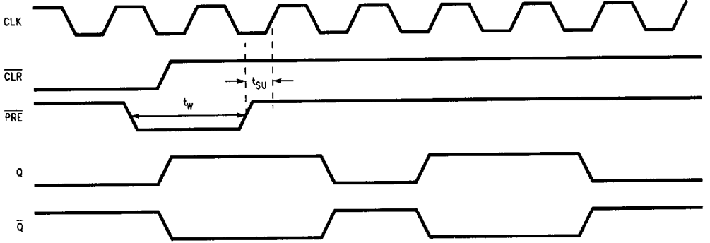
Minimum Skew Divide-by-2 Clock Drivers CGS64/74B304
