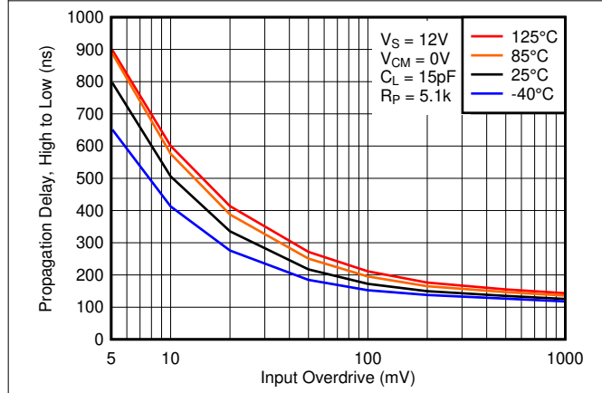
Figure 6-27. High to Low Propagation Delay vs. Input Overdrive Voltage, 12V
