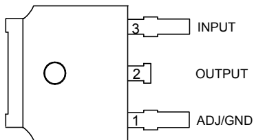
(TO-252-2 (3))
