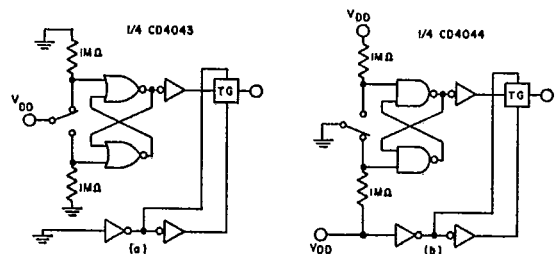
Fig. 13 - Switch bounce eliminator.
