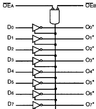
IDT54/74FCT540/541
