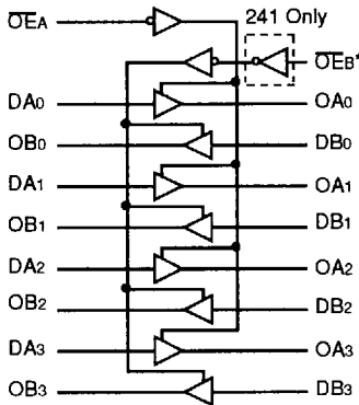
IDT54/74FCT241/244
