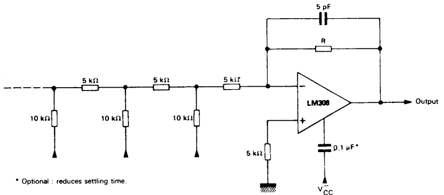
D/A CONVERTER USING LADDER NETWORK
