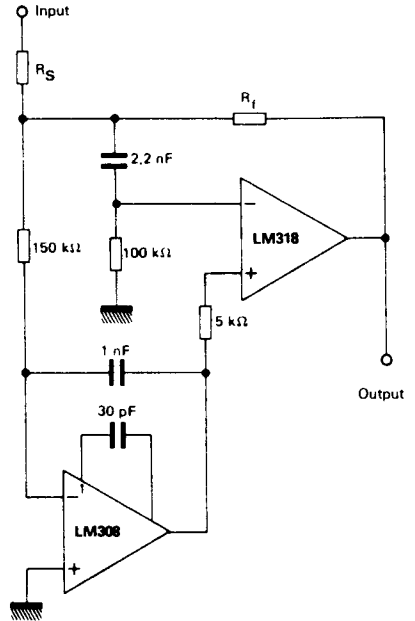
FAST SUMMING AMPLIFIER WITH LOW INPUT CURRENT
