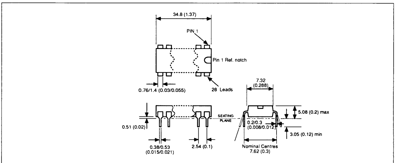
Figure 17. 28 plastic DIL Package (0.3in) DPB
