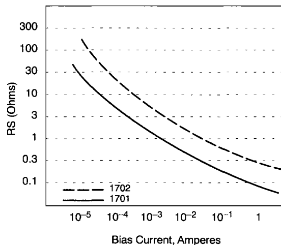
Typical Forward Resistance vs. Bias Current
