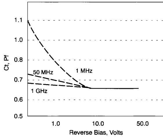
Typical Capacitance
