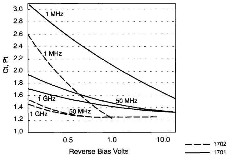
Typical Capacitance Voltage Variation
