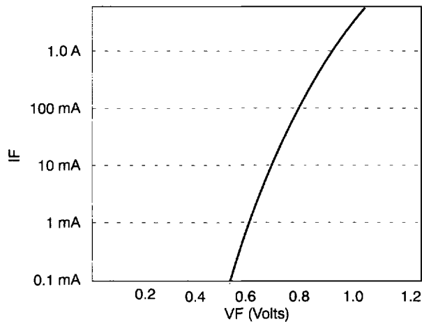
DC Characteristics
