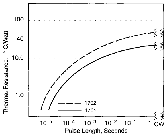
Thermal Resistance
