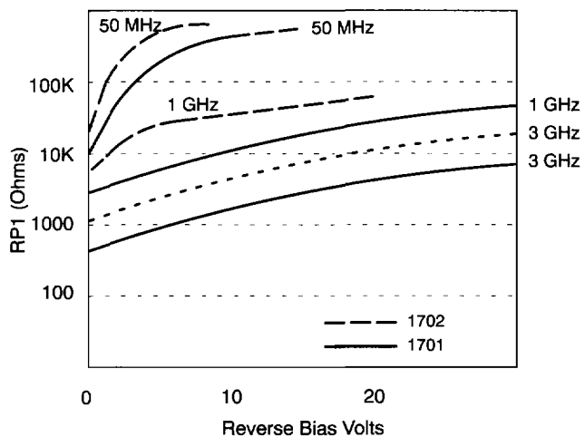
Parallel Resistance RP
