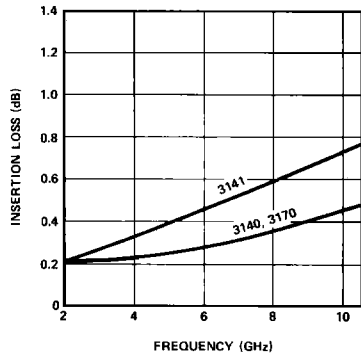
Figure 2. Typical Insertion Loss vs. Frequency.
