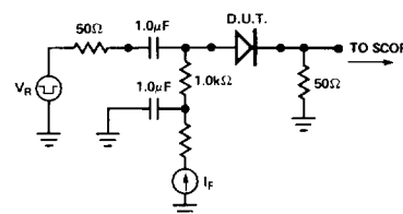
Figure 7. Basic t_{rr} Test Setup.
