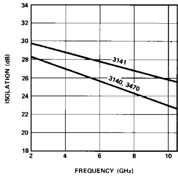
Figure 4. Typical Isolation vs. Frequency.
