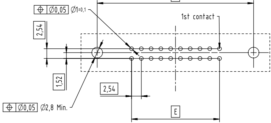
PC-Board layout view component side thickness 1,6 mm
