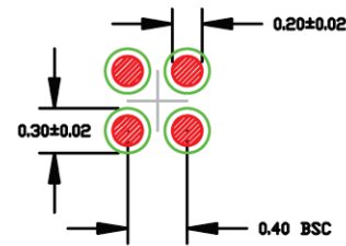
RECOMMENDED LAND PATTERN NOTE: 3,4
