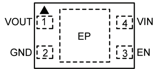
4-Pin 1.2mm × 1.6mm Thin DFN (MT) Top View
