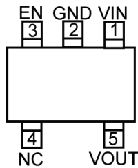
5-Pin SOT-23 (M5) Top View
