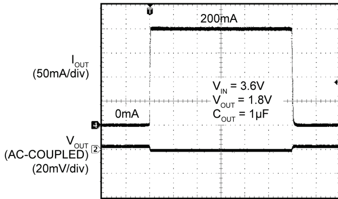
Load Transient (0mA to 200mA)
