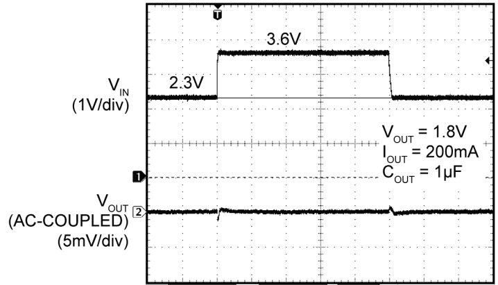
Line Transient (2.6V to 3.6V)
