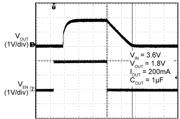
Enable Turn-Off
