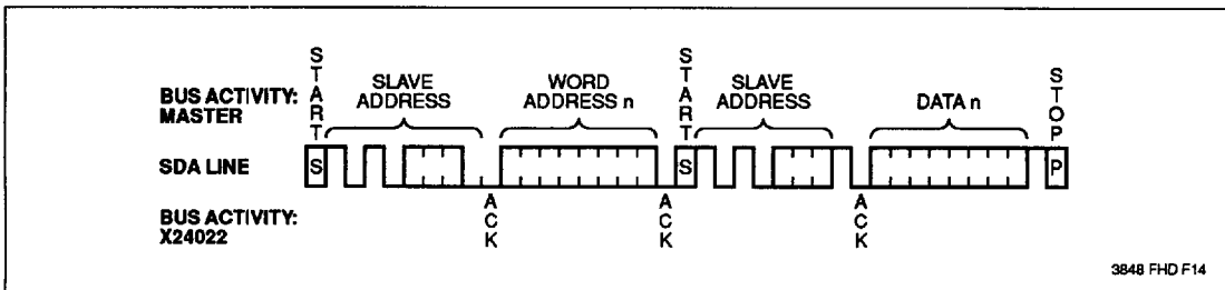
Figure 8. Random Read
