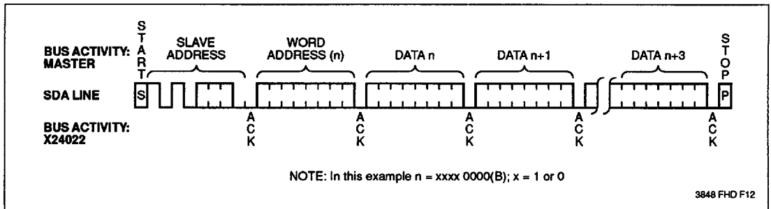
Figure 6. Page Write
