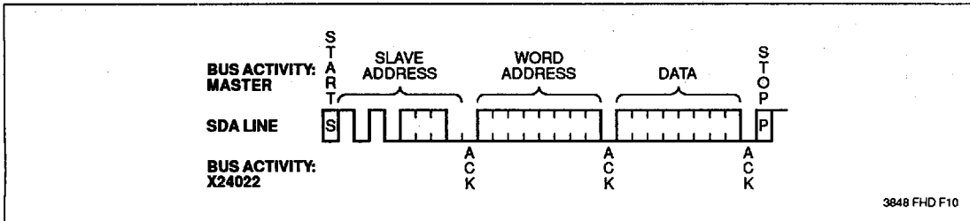
Figure 5. Byte Write
