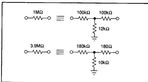
FIGURE 6. Equivalent Resistances.
