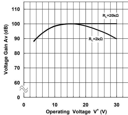
Voltage Gain vs. Operating Voltage ( T_a=25^\circ C )
