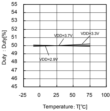
Fig.39 18.4MHz Temperature-Duty
