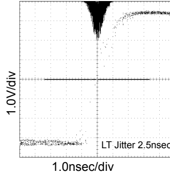
Fig62. 22.6MHz LT Jitter VDD=3.3V, at CL=15pF
