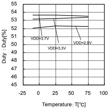
Fig.42 27MHz Temperature-Duty
