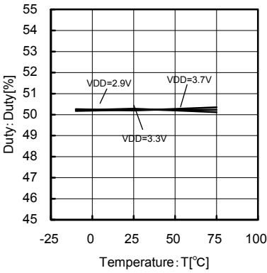
Fig.36 16.9MHz Temperature-Duty
