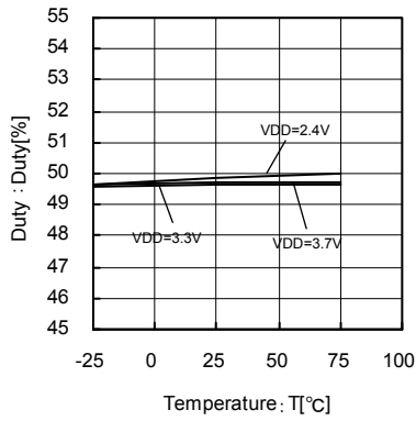
Fig.72 24.6MHz Temperature-Duty
