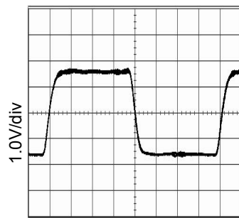
Fig.88 24.6MHz output waveform VDD=3.3V, at CL=15pF
