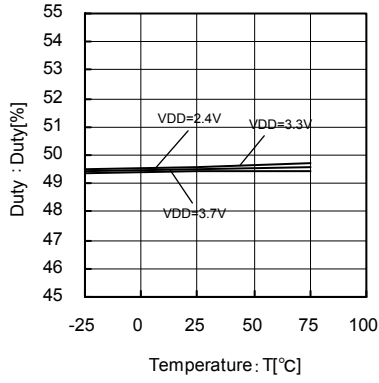
Fig.69 33.9MHz Temperature-Duty
