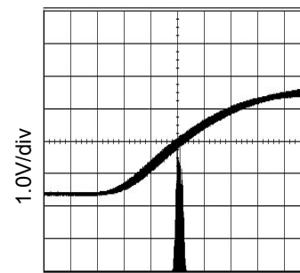
Fig.89 24.6MHz Period-Jitter VDD=3.3V, at CL=15pF
