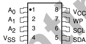
TSSOP Package (U, Y, GY)
