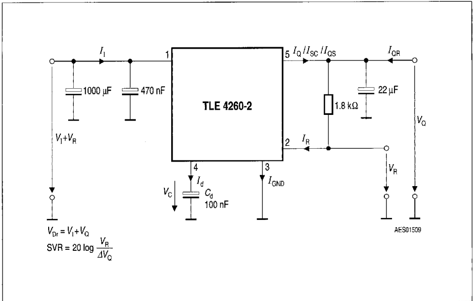
Test Circuit
