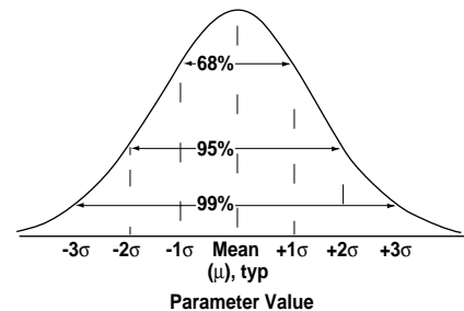
Figure 21. Normal Distribution.
