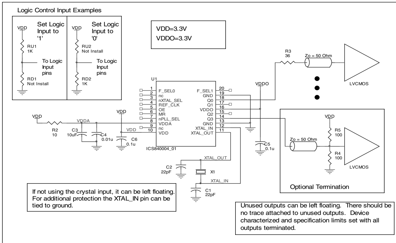
FIGURE 4. ICS840004-01 SCHEMATIC EXAMPLE
