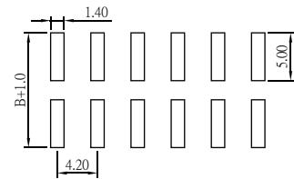
Recommended PCB Layout (PCB TOLERANCE ±0.05)
