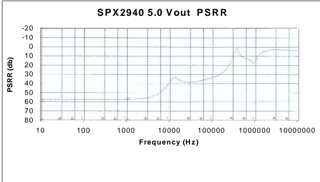
Figure 20. 5Vout PSRR. Vin=10V, Vout=5V, Cout=22uF, Iout=10mA.
