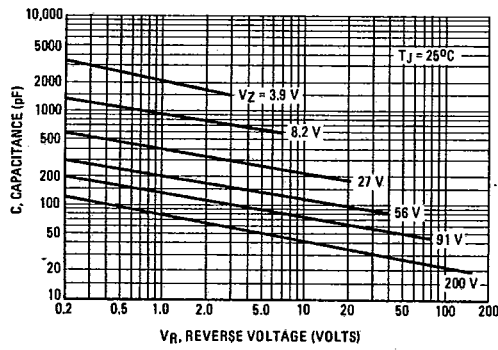
FIGURE 10 - TYPICAL CAPACITANCE
