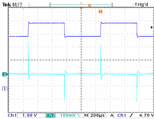
Load Transient (I OUT =1mA-100mA)
