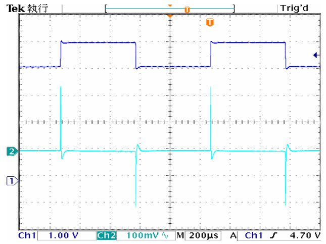
Line Transient (I OUT =200mA, V IN =4V-5V)
