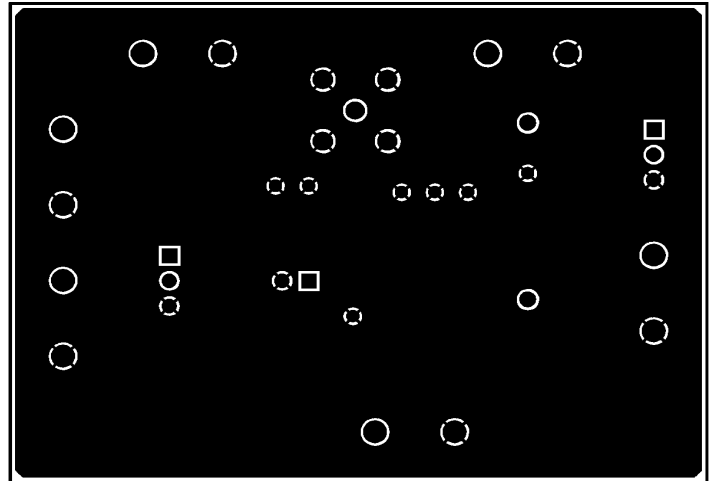
Bottom Copper
