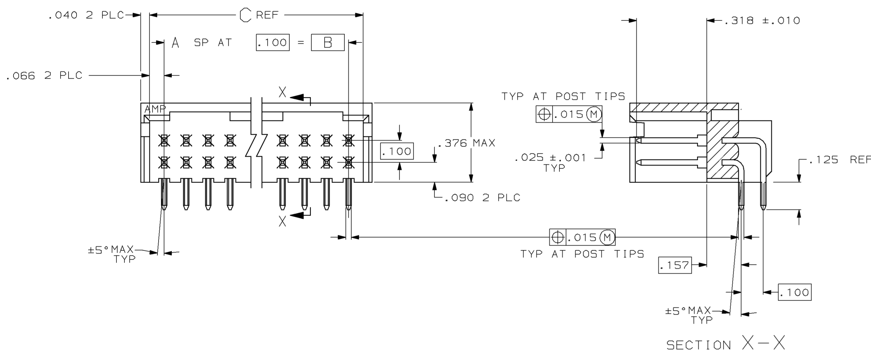
SECTION X-X
