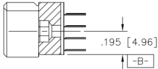
SECTION U-U
