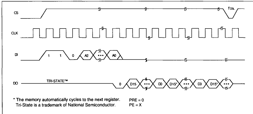
FIGURE 14-2: READ TIMING
