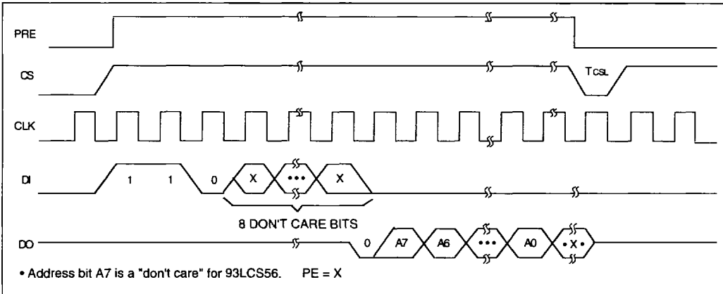
FIGURE 14-10: PREN TIMING
