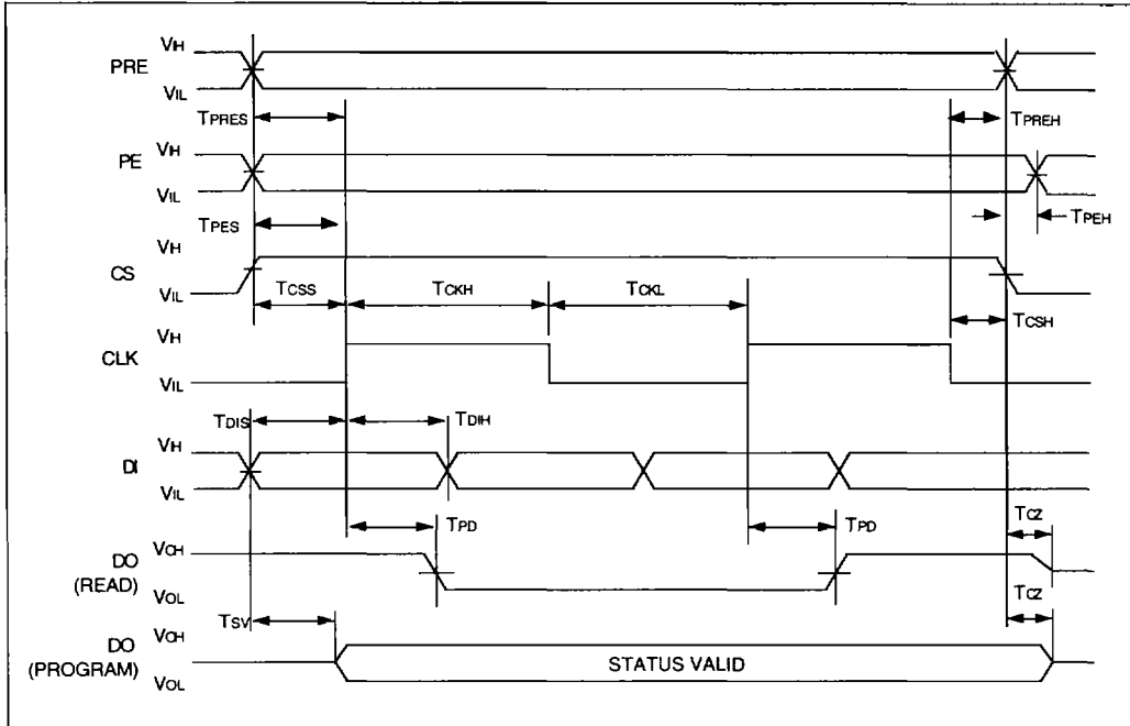
FIGURE 14-2: READ TIMING
