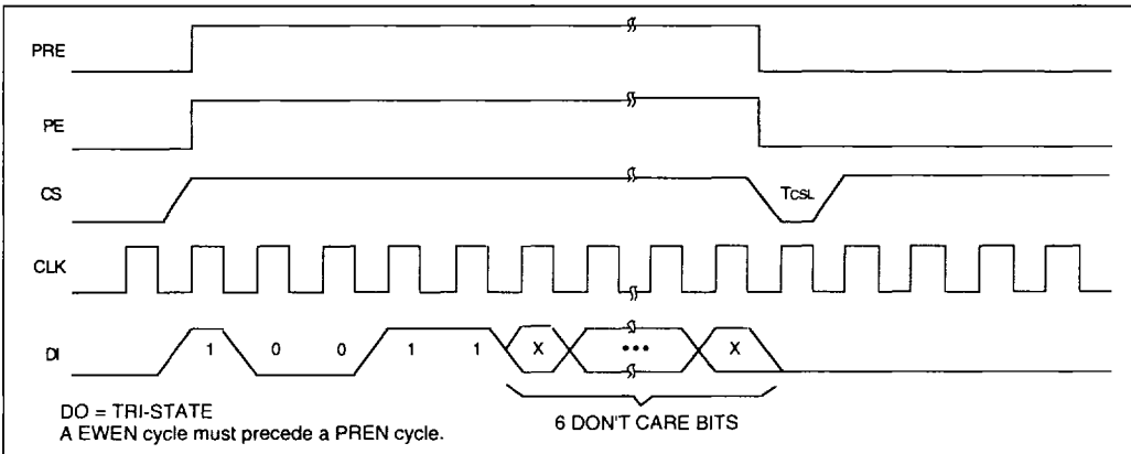
FIGURE 14-10: PREN TIMING
