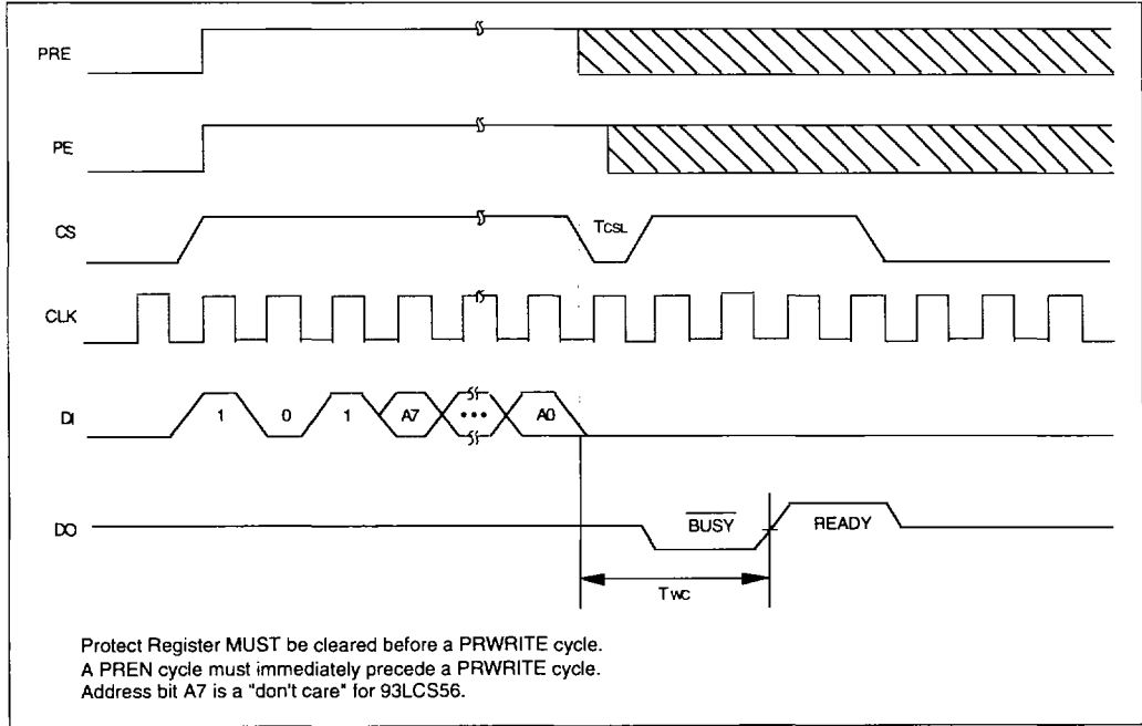
FIGURE 14-12: PRWRITE TIMING
