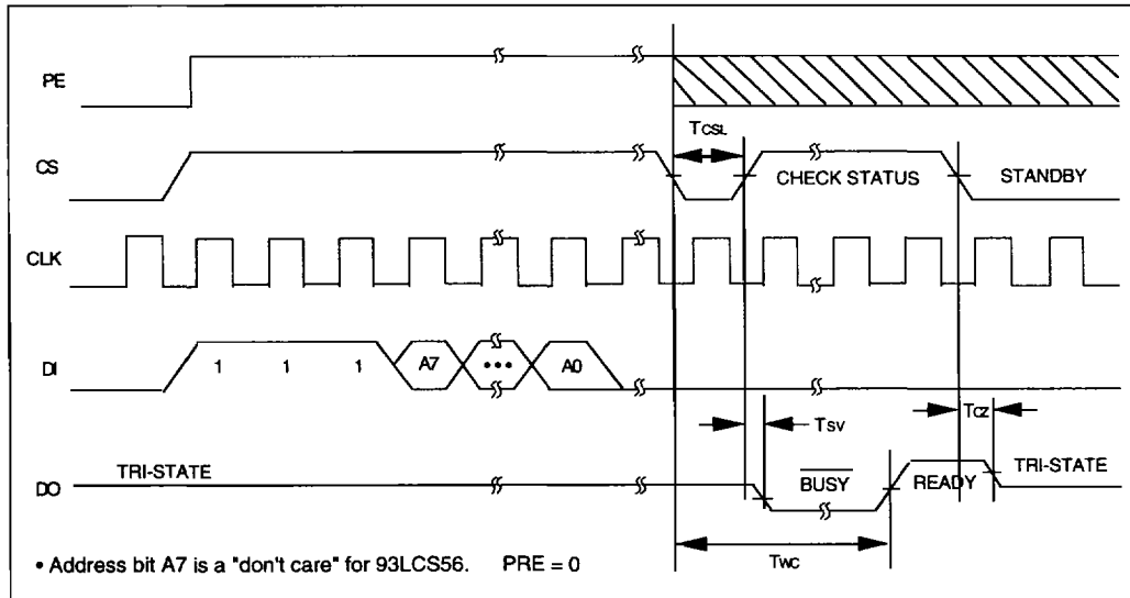
FIGURE 14-7: ERASE TIMING
