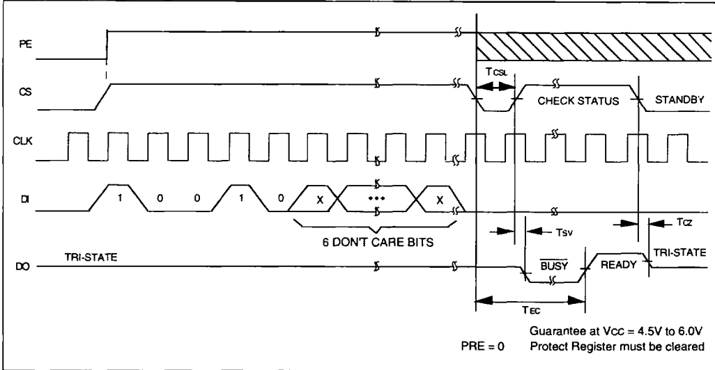
FIGURE 14-9: PPREAD TIMING
