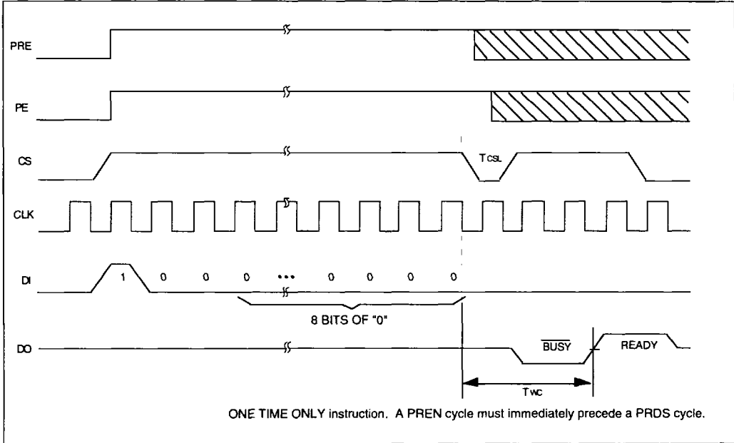
FIGURE 14-13: PRDS TIMING
