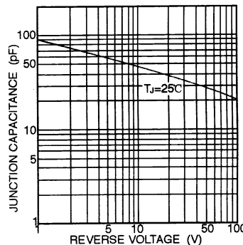
FIG. 4-TYPICAL JUNCTION CAPACITANCE
