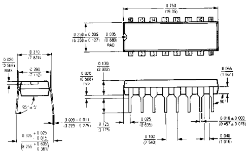
16 Pin Molded DIP (N)
