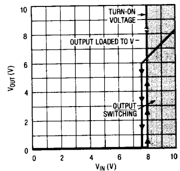
LT1525A Start-Up
