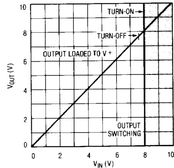
LT1527A Start-Up
