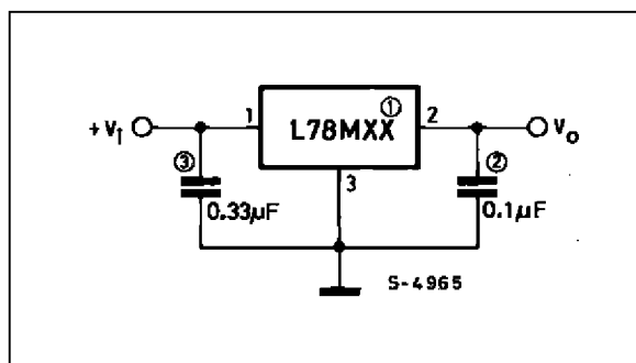
Figure 13 : Fixed Output Regulator.
