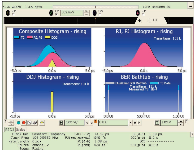
Figure 2: Jitter Analysis of a QT84L-106.25MHZ
