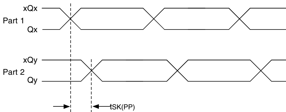
Part-to-Part Skew
