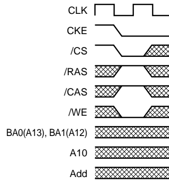
Deep power down entry command
