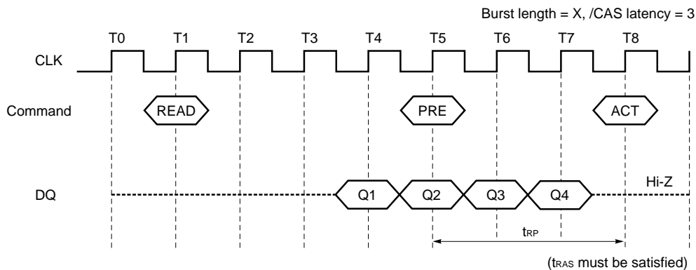
Precharge Termination in READ Cycle (CL = 3)
