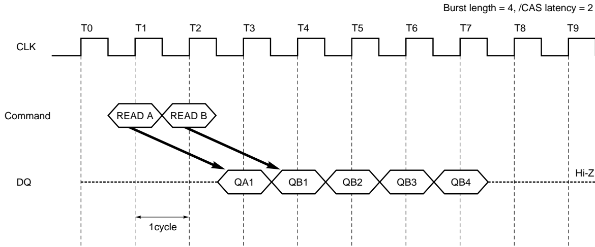
Read to Read Command Interval
