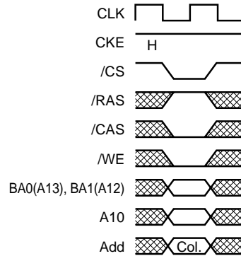
Write command
