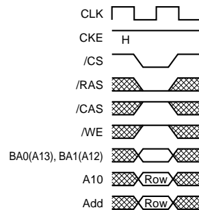
Activate command
