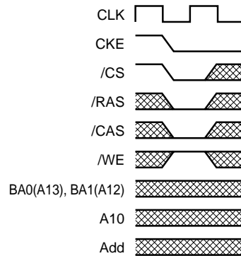
Self refresh entry command
