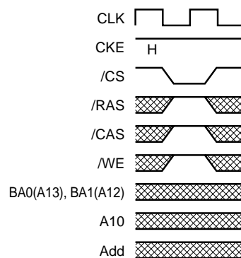
No operation
