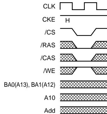
Auto refresh command
