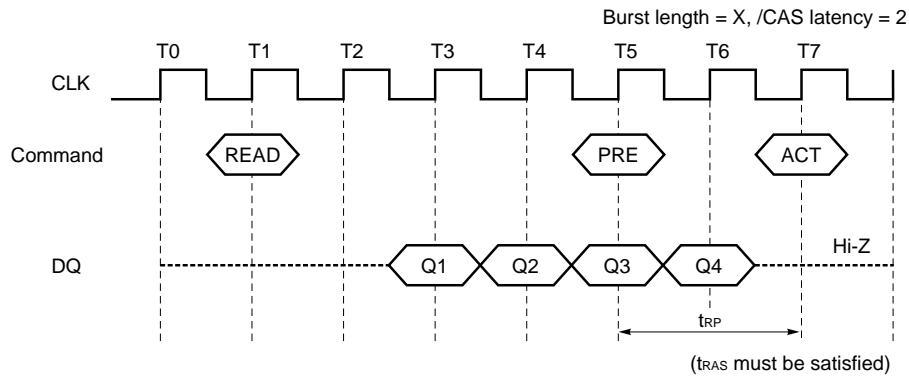
Precharge Termination in READ Cycle (CL = 2)
