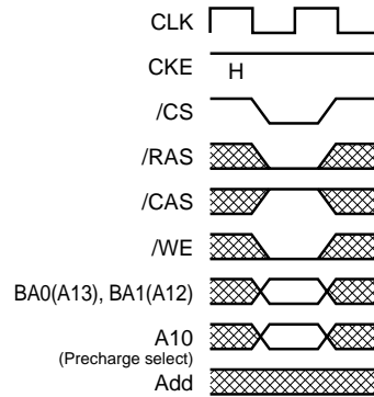
Precharge command
