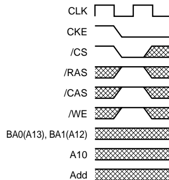
Power down entry command
