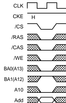
Extended Mode register set command
