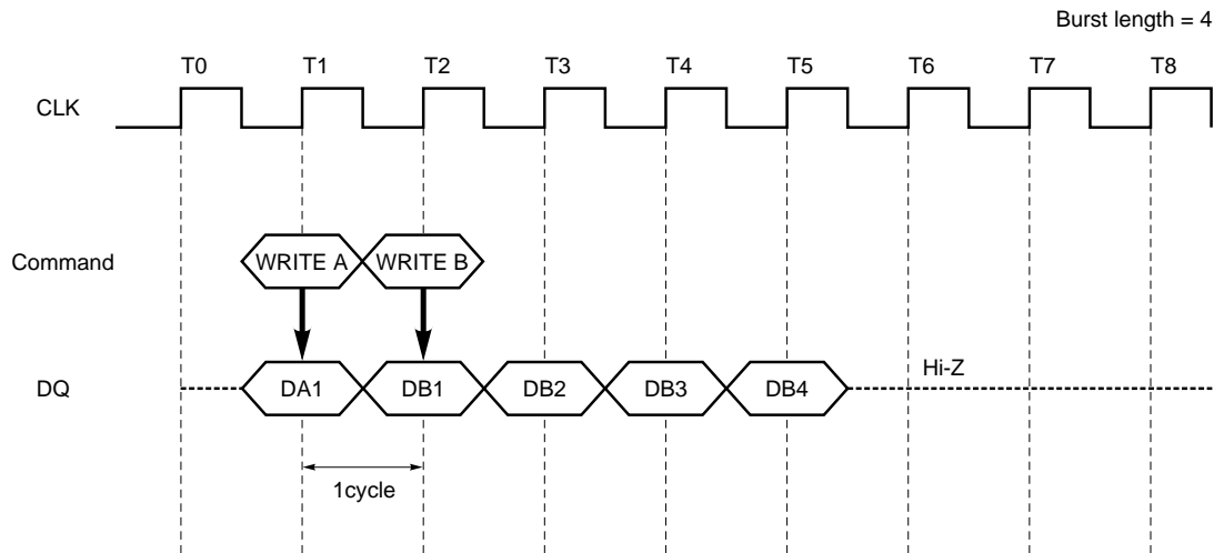
Write to Write Command Interval
