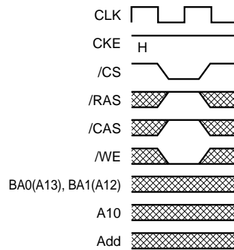
Burst stop command
