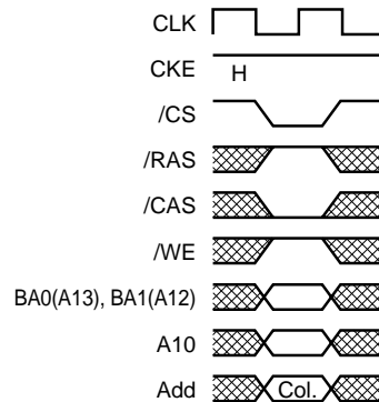
Read command
