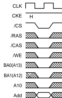
Mode register set command
