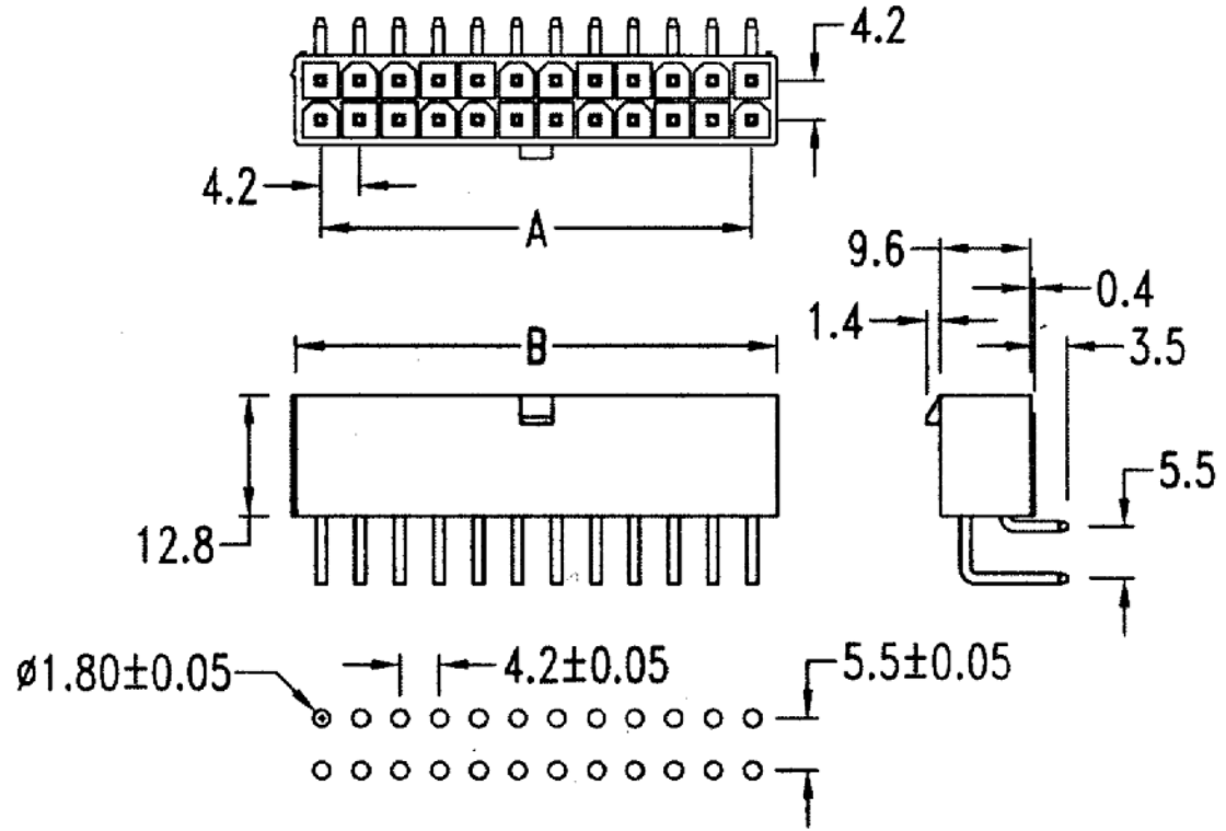
PC Board Hole Layout and Dimensions
