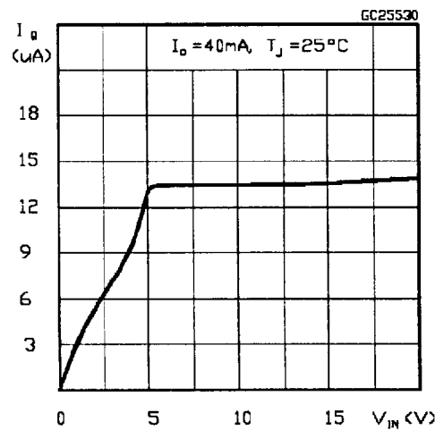
Figure 5: Quiescent Current
