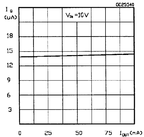
Figure 6: Quiescent Current
