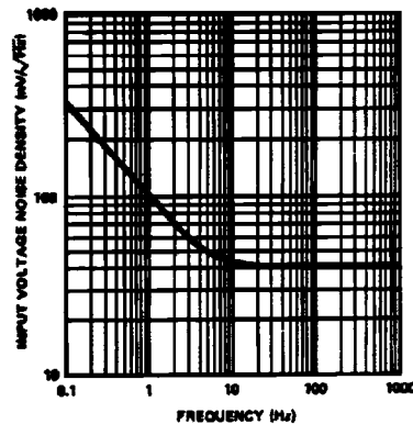
INPUT VOLTAGE NOISE DENSITY (en) vs FREQUENCY
