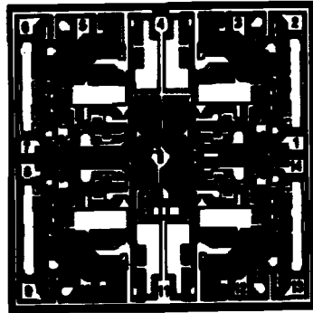
DIE SIZE 0.083 × 0.087 inch, 8091 sq. mils (2.36 × 2.21 mm, 5.22 sq. mm)
