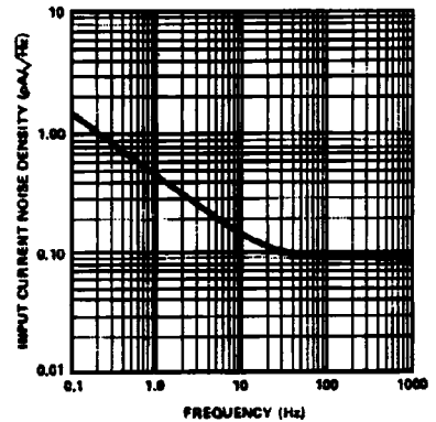
INPUT CURRENT NOISE DENSITY (in) vs FREQUENCY
