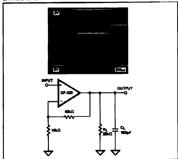
LARGE-SIGNAL TRANSIENT RESPONSE
