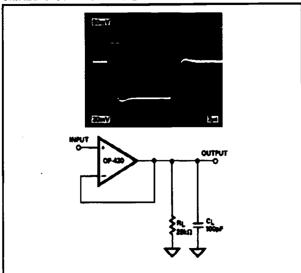
SMALL-SIGNAL TRANSIENT RESPONSE
