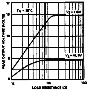
MAXIMUM OUTPUT VOLTAGE vs LOAD RESISTANCE
