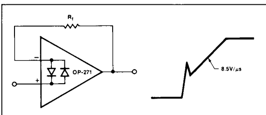
FIGURE 2: Pulsed Operation
