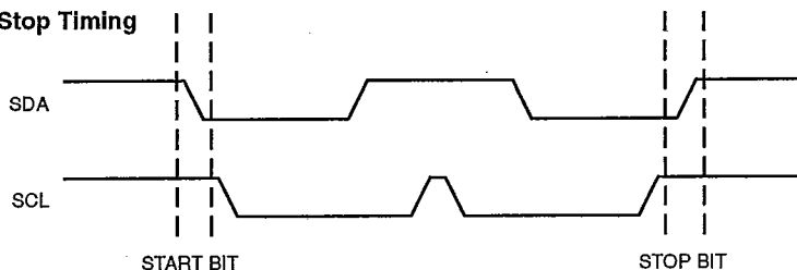
Figure 3. Start/Stop Timing
