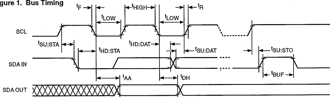
Figure 1. Bus Timing
