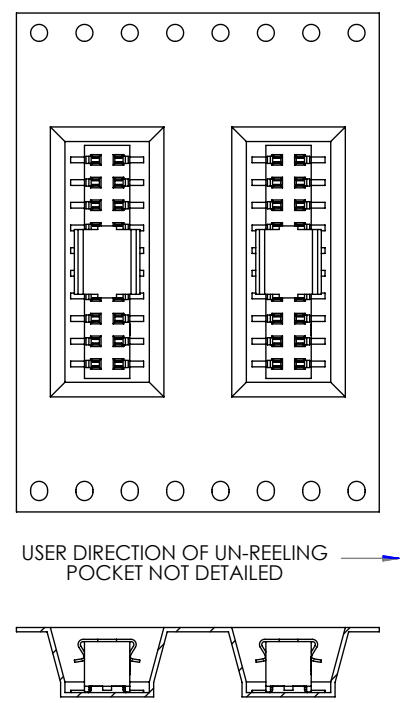
FIG 8 -TR: TAPE & REEL PACKAGING
