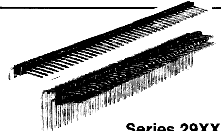
Series 29XX 90° Squarestix Header 1-50 Pin Single Row 2-100 Pin Dual Row
