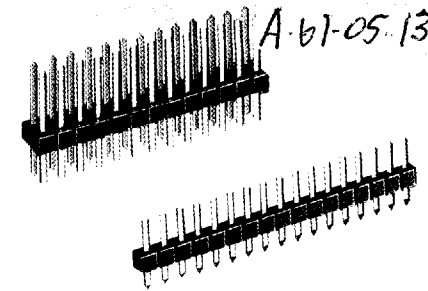
Series 29XX 2MM Squarestix Header 1-50 Pin Single Row 2-100 Pin Dual Row
