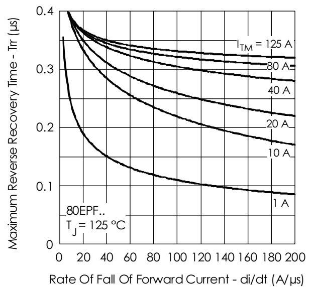
Fig. 9 - Recovery Time Characteristics, T_J = 125^\circ\text{C}
