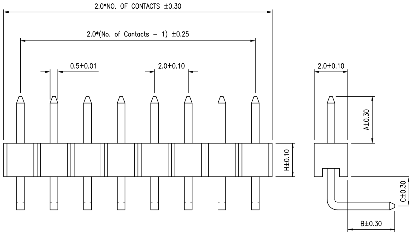
Pin Chart
