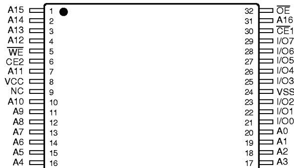
32-Pin TSOP-I
